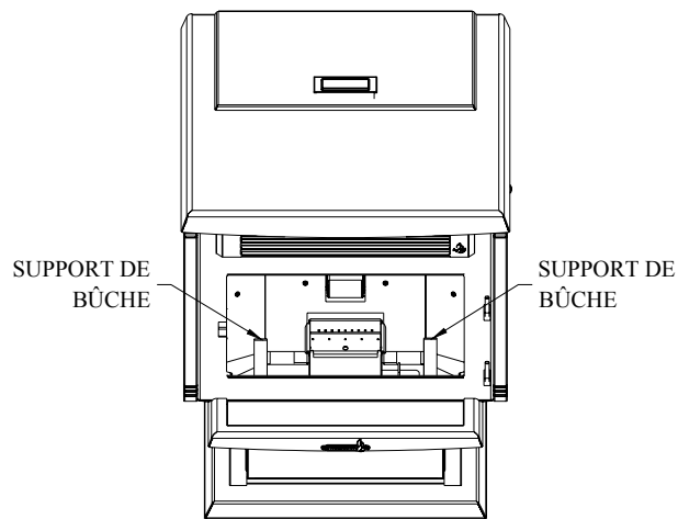
Figure 14c Localisation des supports
