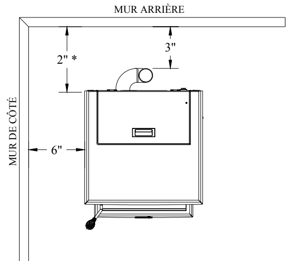
*INSTALLATION HORIZONTALE
