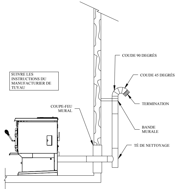
FIGURE 7 Évacuation murale
