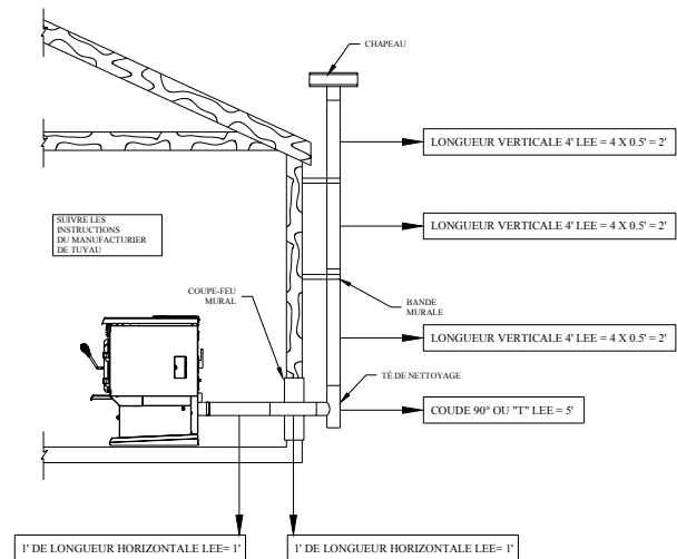
FIGURE 8 Évacuation murale
