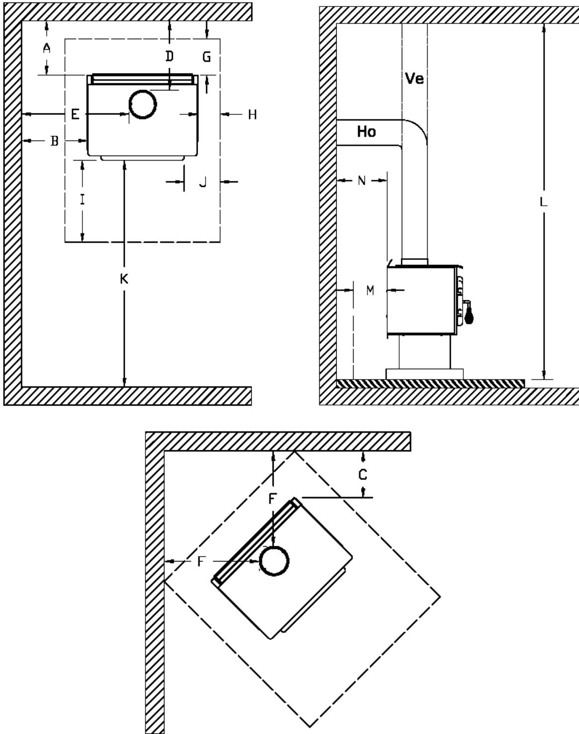
FIGURE 2.3 Clearances to combustibles and floor protection
